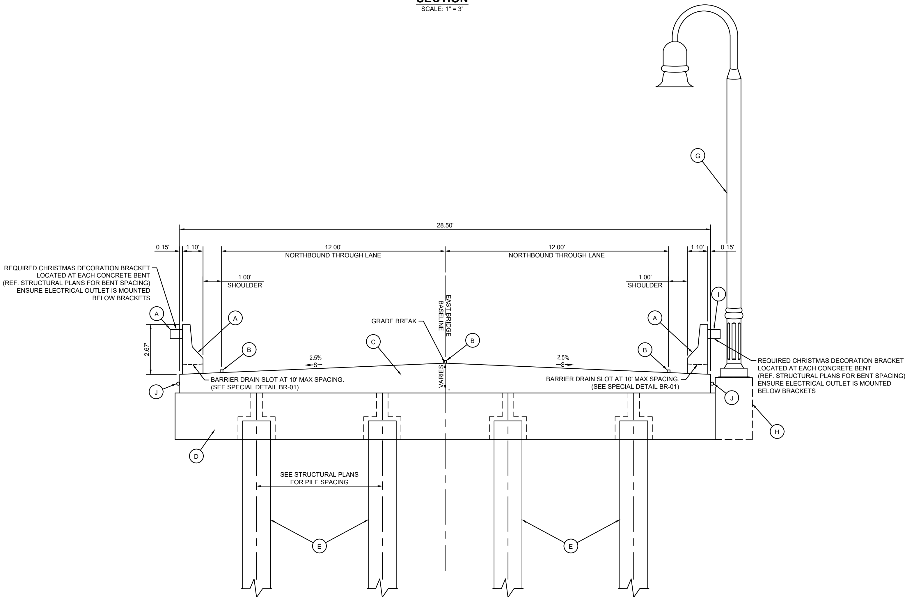
EAST BRIDGE TYPICAL SECTION SCALE: 1" = 3'
