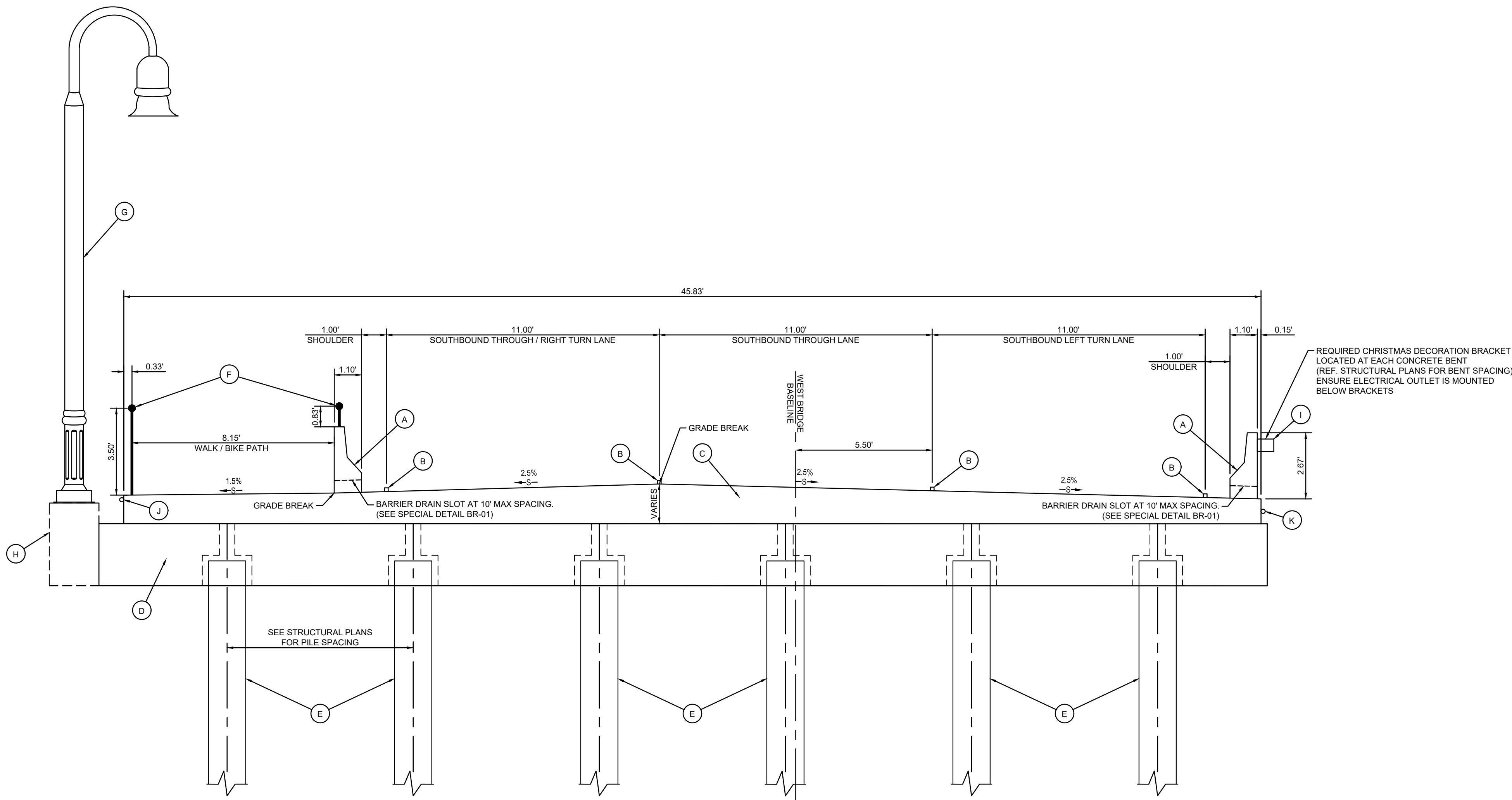
WEST BRIDGE TYPICAL SECTION SCALE: 1" = 3'
